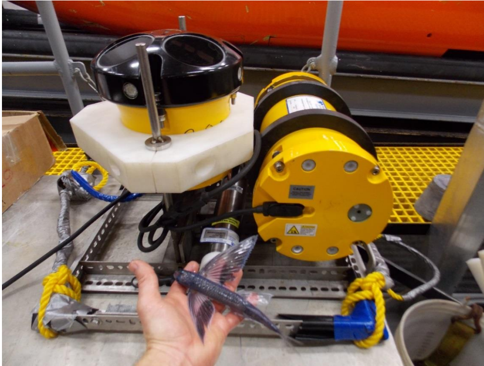
1) Fixed bottom mount with 600kHz TRDI WH Monitor ADCP, external battery case, and SBE-37 MicroCAT (salinity/temperature/pressure recorder).
