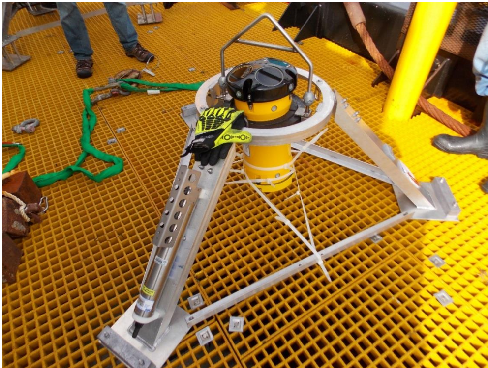
2) Gimbaled tripod with 300kHz TRDI Workhorse Sentinel ADCP and SBE-37 MicroCAT (salinity, temperature, pressure recorder).
