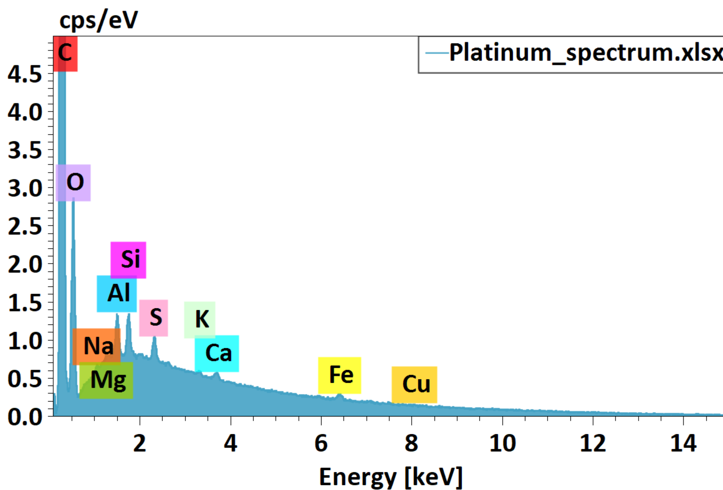
Platinum_spectrum.xlsx
